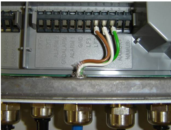
9: Tighten the nut and insert the cores into the terminal clamps
